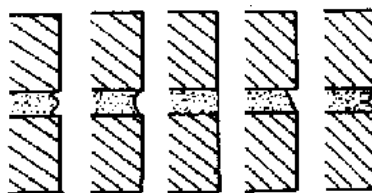
Examples of appropriate mortar joints.
